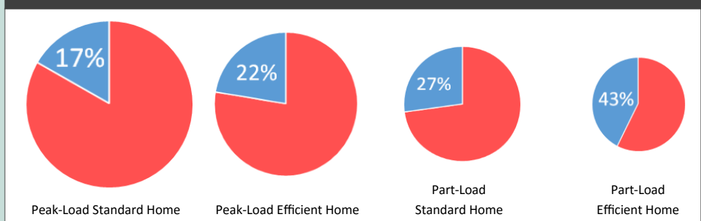
Figure 1. Latent Loads Increase as a Percentage of Total Loads at Part-Load Conditions.
