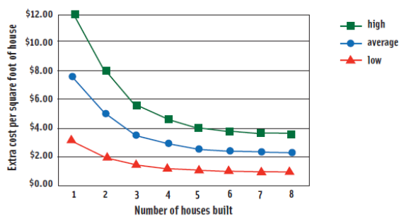
Declines in Wall Cost with Crew Experience
