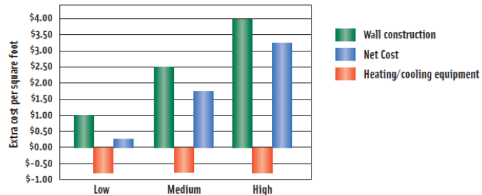
Total Costs of Construction with ICFs
