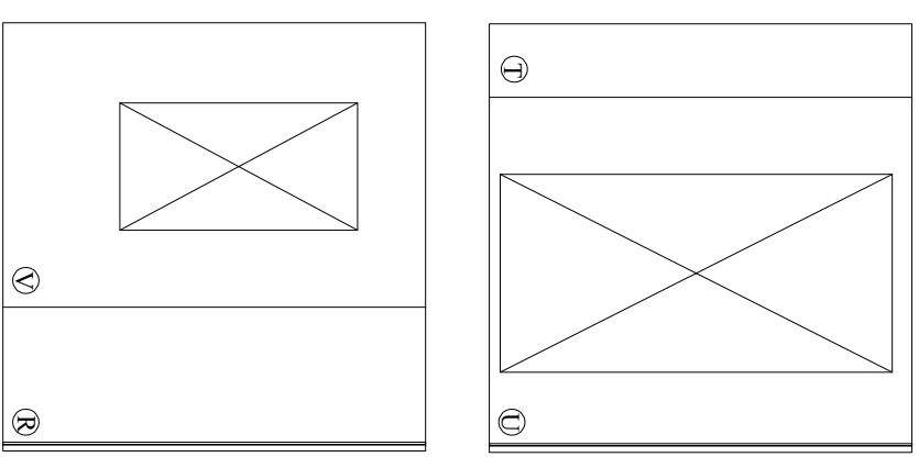
Figure 11. Cutting plan for the Front and Rear wall sheathing
