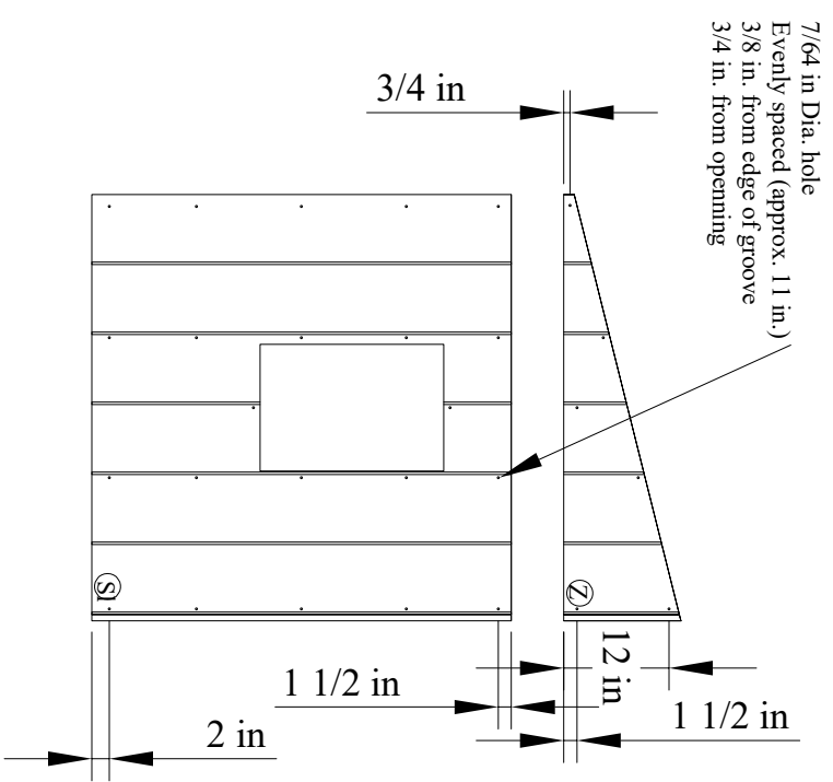
Figure 13d. Drilling plan for Left wall sheathing
