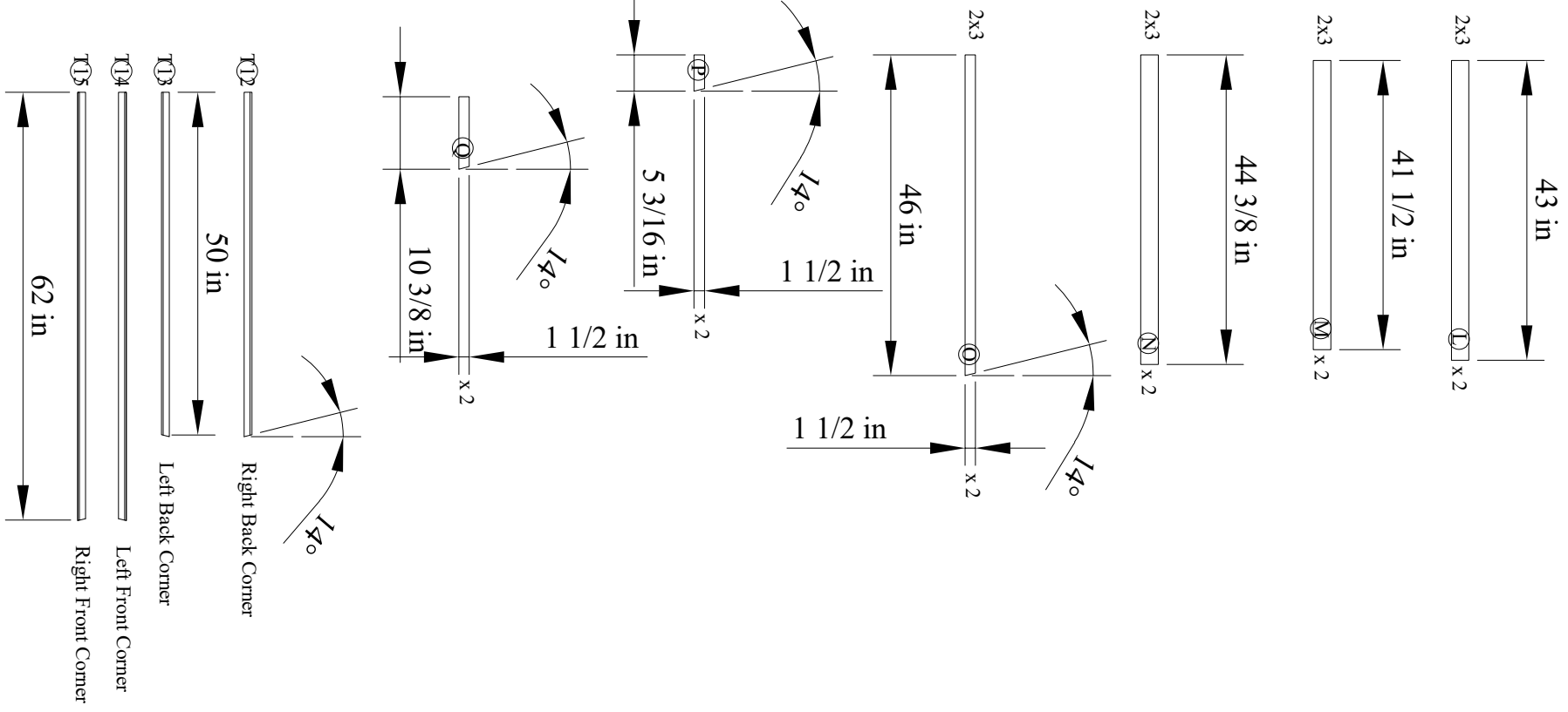
Figure 1b. Wall framing members
