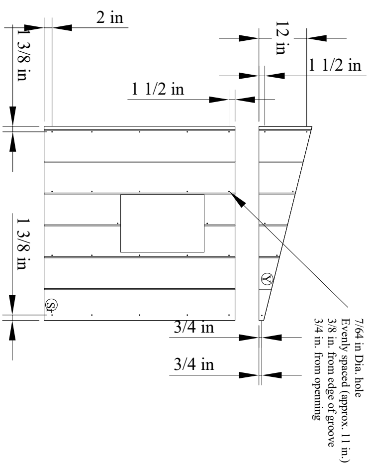
Figure 13c. Drilling plan for Right wall sheathing
