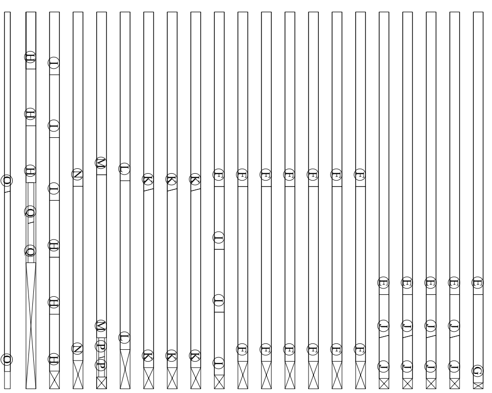
Figure 5. Cutting plan for wall framing
