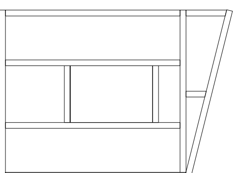
Figure 21c. Right wall framing assembly
