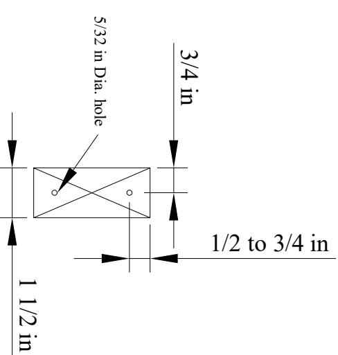
Figure 3. Marking and drilling plan for Floor framing
