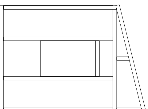
Figure 21d. Left wall framing assembly
