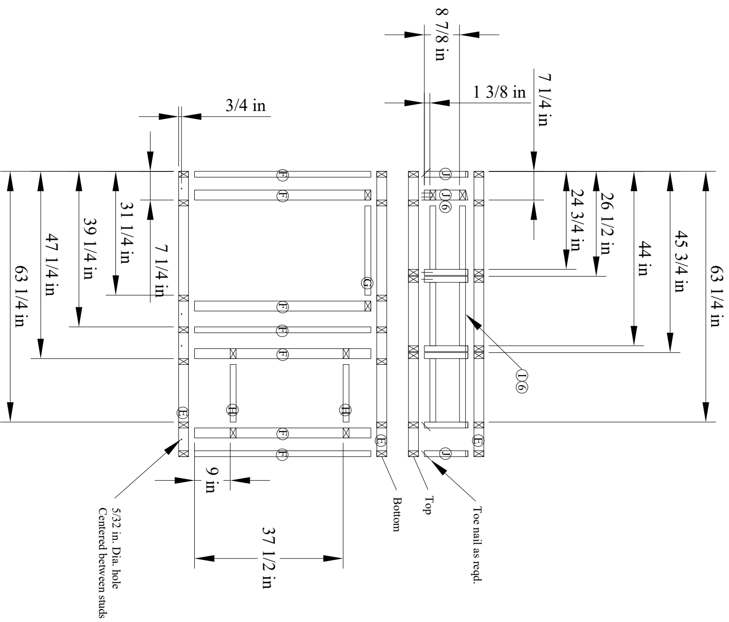
Figure 21d. Left wall framing assembly
