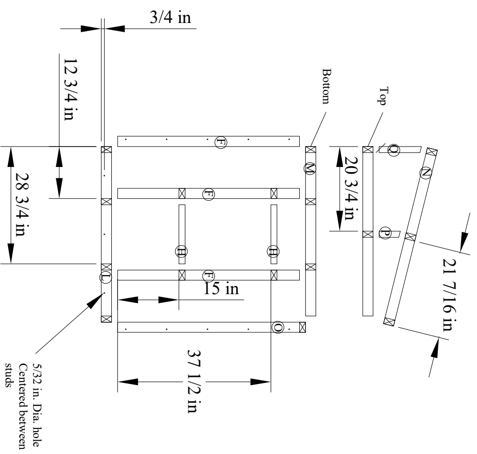
Figure 6c. Marking and drilling plan for Right Wall framing
