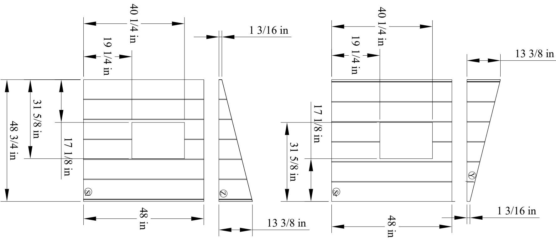
Figure 1c. Wall sheathing panels
