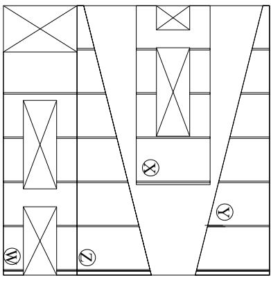
Figure 12. Cutting plan for the top portions of Front, Right and Left wall sheathing
