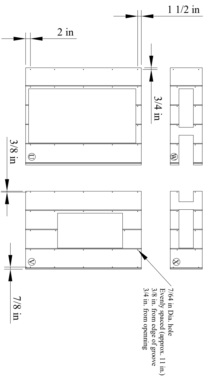
Figure 13a. Drilling plan for Front wall sheathing
