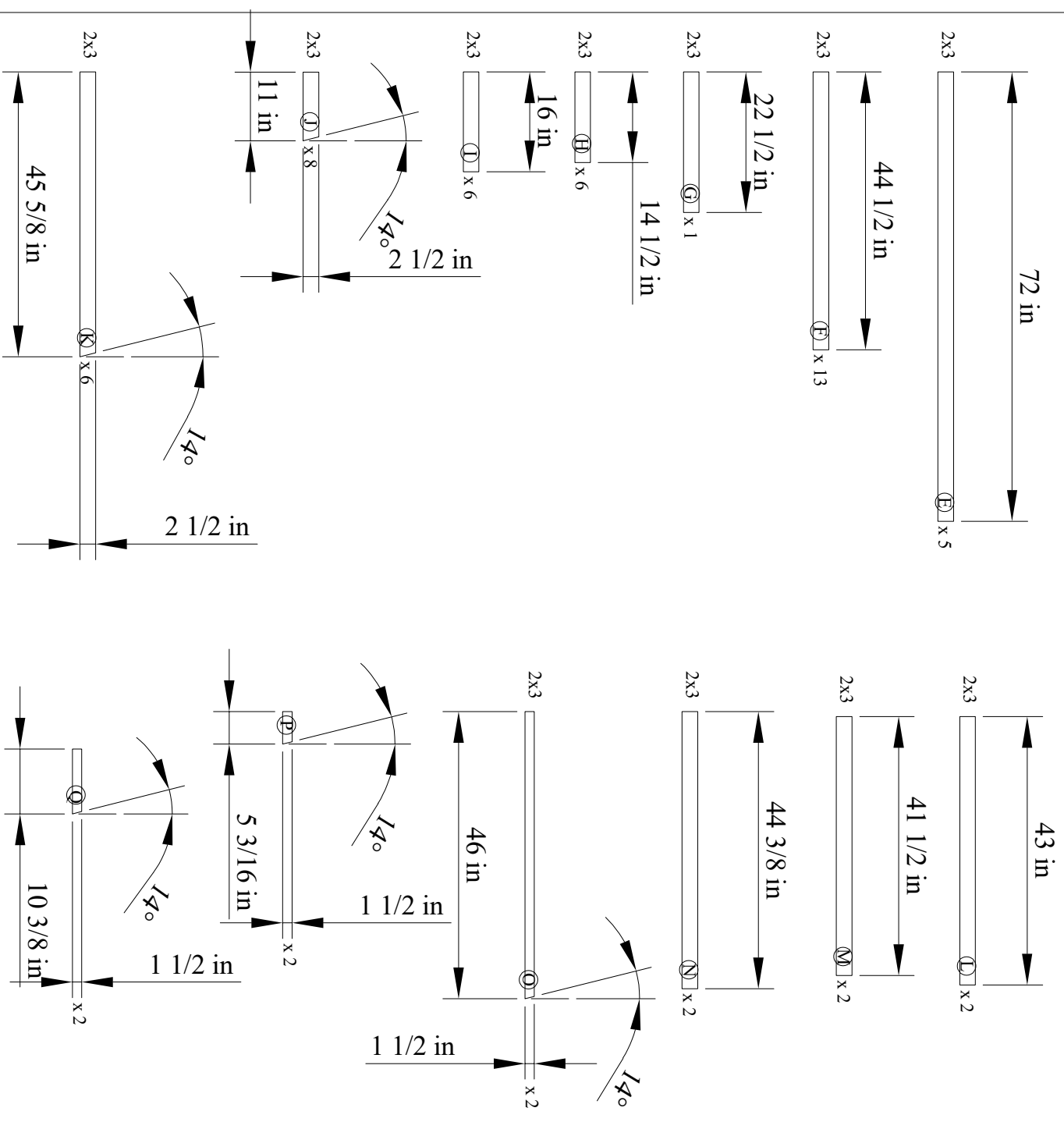
Figure 1b. Wall framing members
