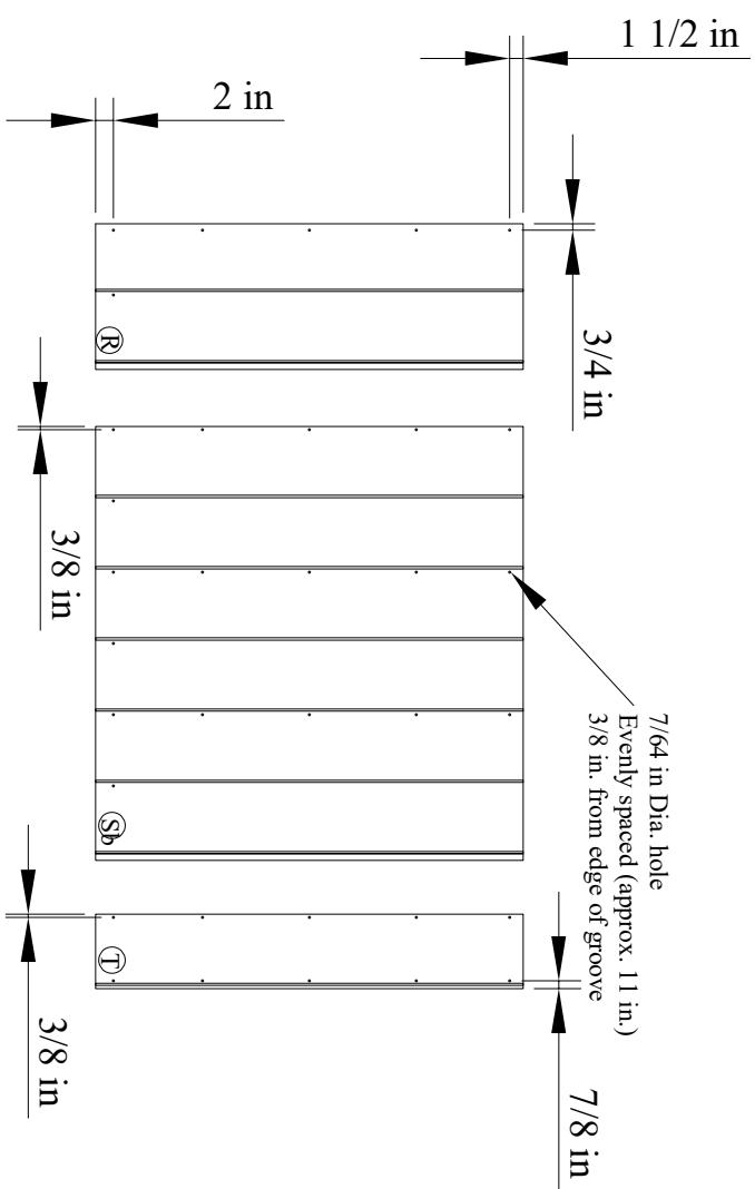
Figure 13b. Drilling plan for Rear wall sheathing
