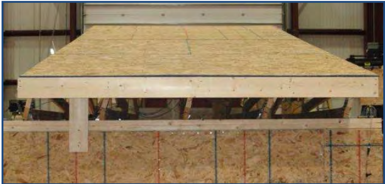
Figure 16 – Specimen C heel rotation at failure
